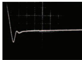
b) with CR snubber (0.01 \mu F, 5.1 \Omega )
