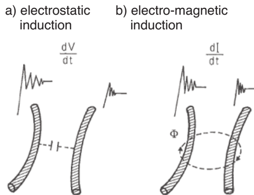
Figure 1. Noise transmission
