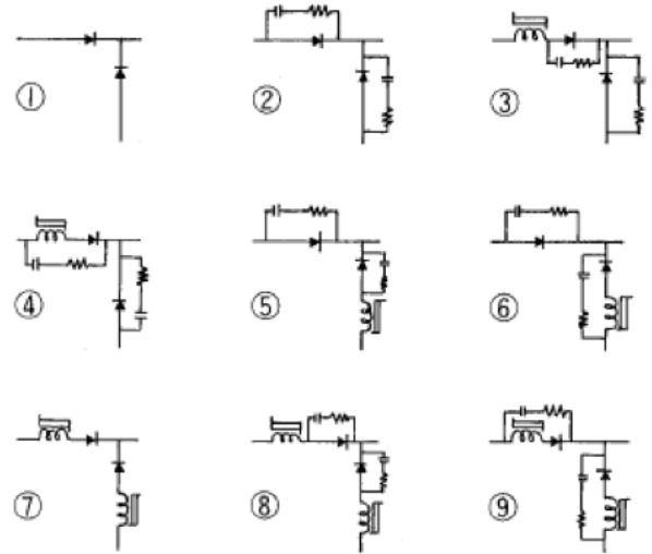
8-2) Combination Of SPIKE KILLER and CR snubber.
